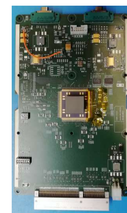
BreadBoard
