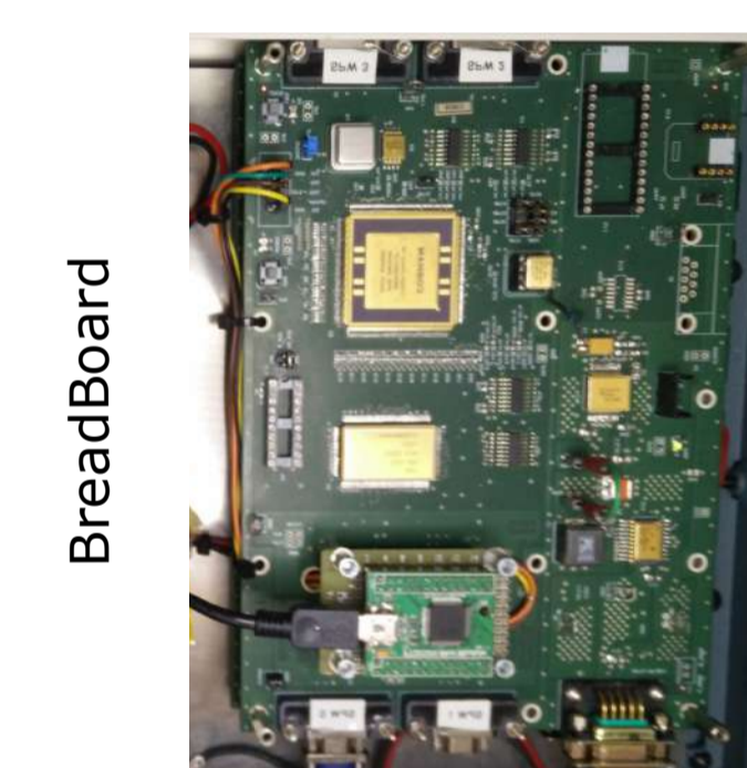
Elegant BreadBoard
