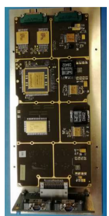
Engineering Model
